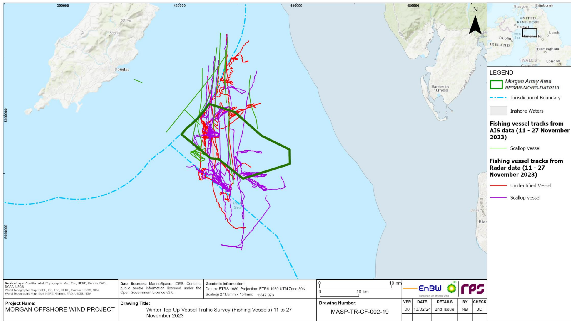
Figure 1.65: AIS fishing vessel track data from 11 to 27 November 2023 66 .
